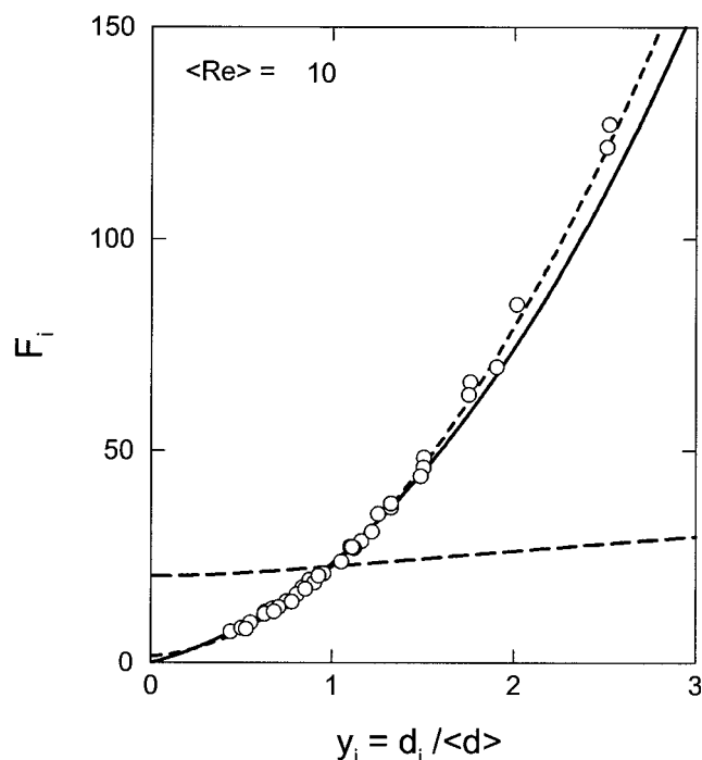
Figure 8. Individual normalized drag force F_i of a bidisperse system as a function of the diameter over the average diameter, for Re = 10 .
