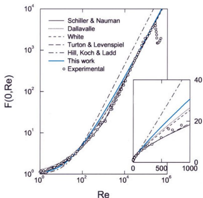
Figure 1. Normalized drag force for an isolated particle as a function of the Reynolds numbers, on a log-log scale.
